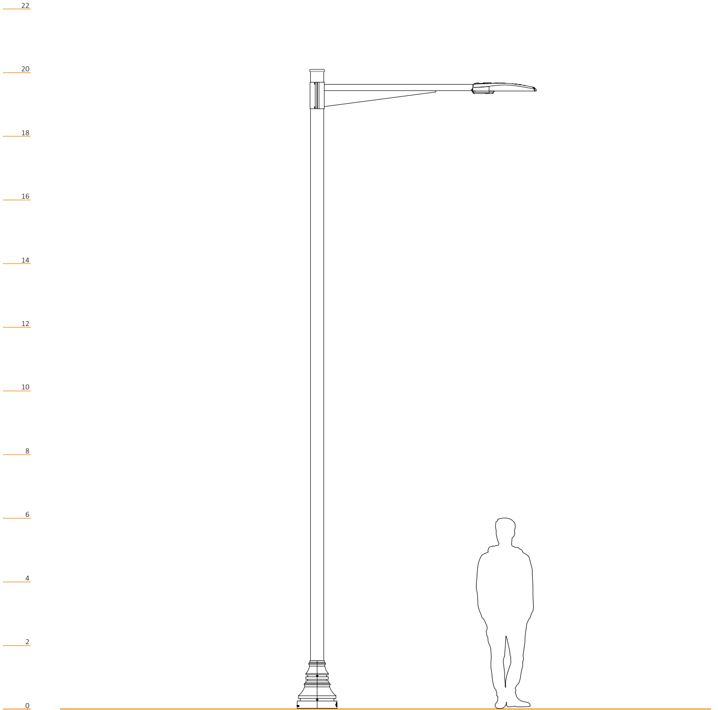
Luminaire: RL Mounting arms: M1A-CF71 Pole: AP05-20 Base cover: WB9-5
